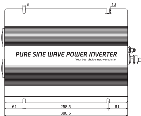
Pure sine wave inverter 2500~3000W
