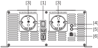
[Pure sine wave inverter 1500~4000W]
